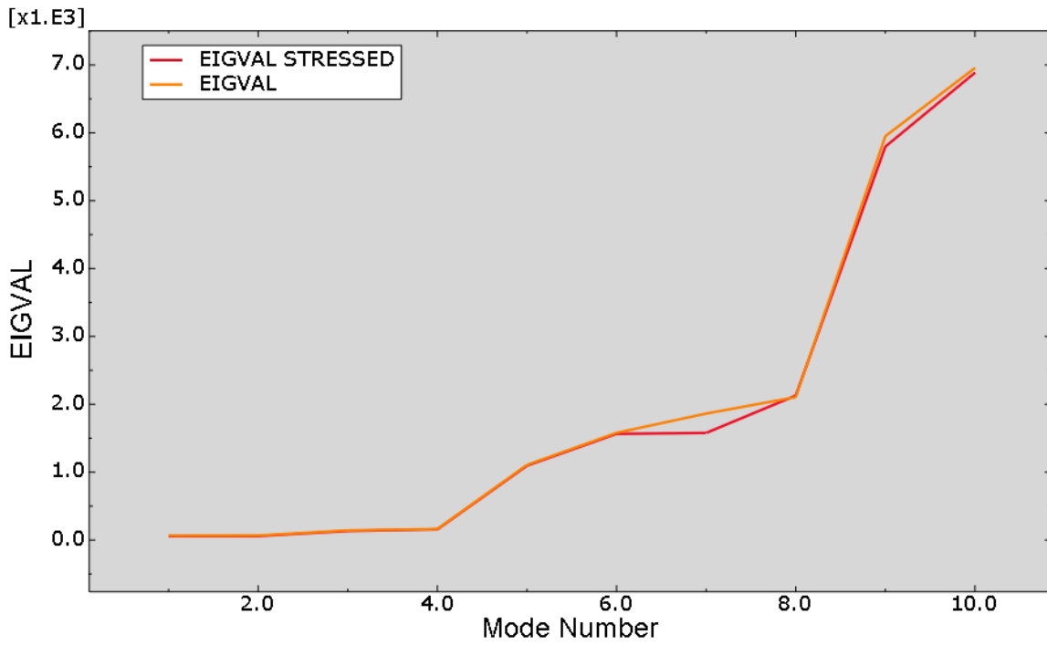
Figure 6. Comparison of natural frequencies in the stressed and non stressed configurations.
